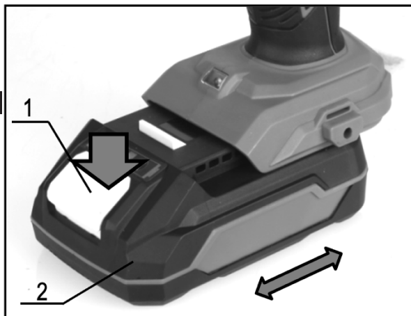
► 1. Button 2. Battery cartridge
